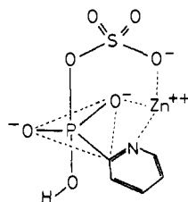
Figure 6. Proposed structure of the intermediate or transition state for the Zn^{2+} catalyzed hydrolysis of 2-pyridylphosphonosulfate (1).
