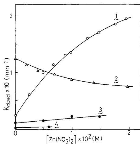
Figure 3. Zn^{2+} ion effects on the hydrolysis rates; see Table II for experimental conditions.
