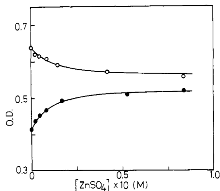
Figure 2. Plots of optical density of the 1 and 2 systems vs. Zn^{2+} ion concentration: (●) [1] = 1 \times 10^{-4} M (260 nm); (○) [2] = 1 \times 10^{-4} M (264 nm); \mu = 1.0 (KCl); pH 5.40; 25 °C.
