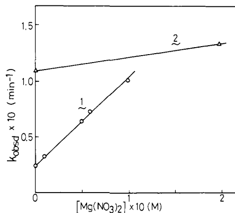
Figure 4. Mg^{2+} ion effects on the hydrolysis rates of 1 and 2; see Table II for experimental conditions.
